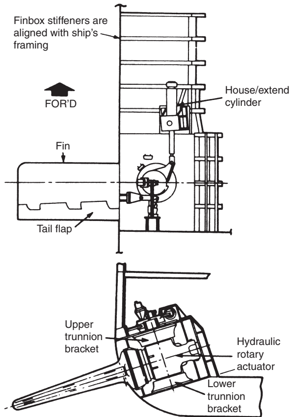
Figure 12.5 Stabilizer fin
