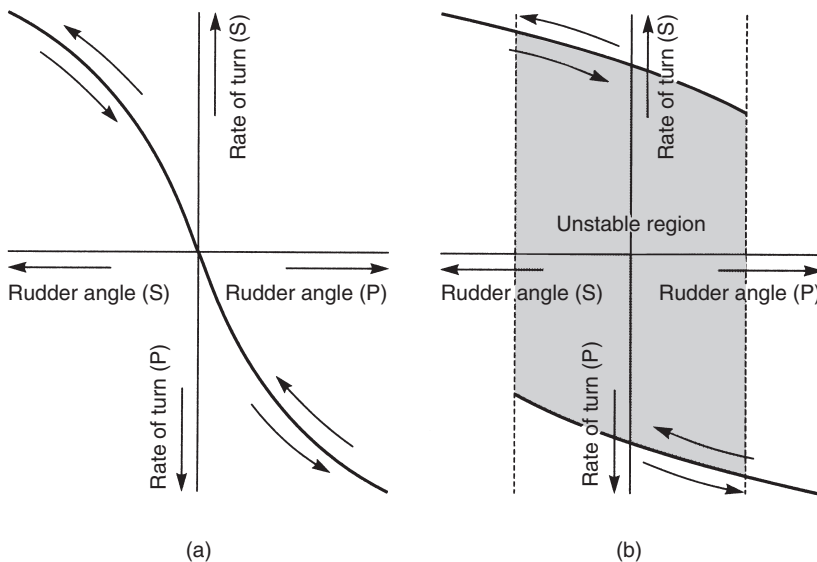
Figure 13.4 Spiral manoeuvre
