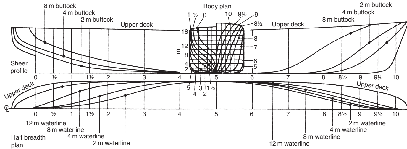
Figure 3.4 Lines plan
