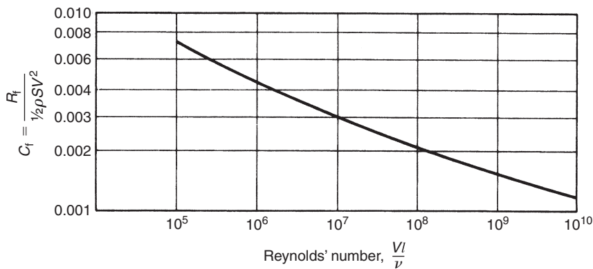
Figure 9.7 Schoenherr line
