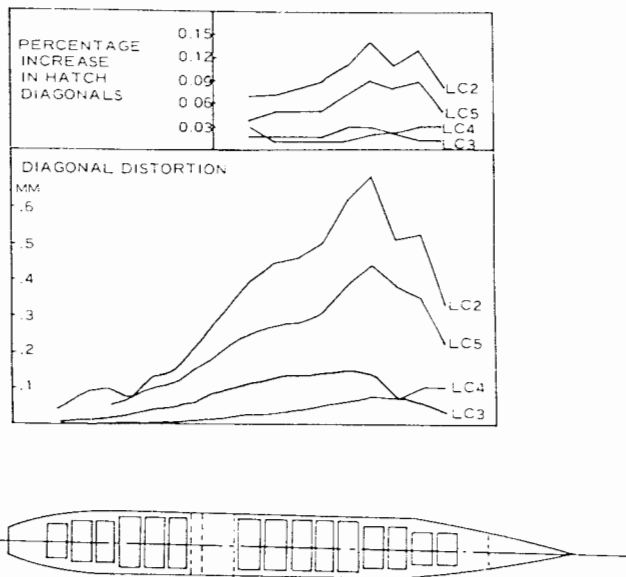
Fig. 48 Hatch diagonal distortion
