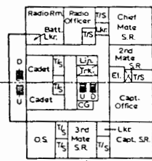
"D" DECK
