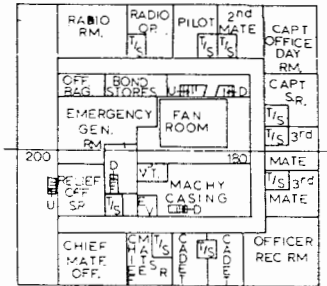
UPPER DECK
