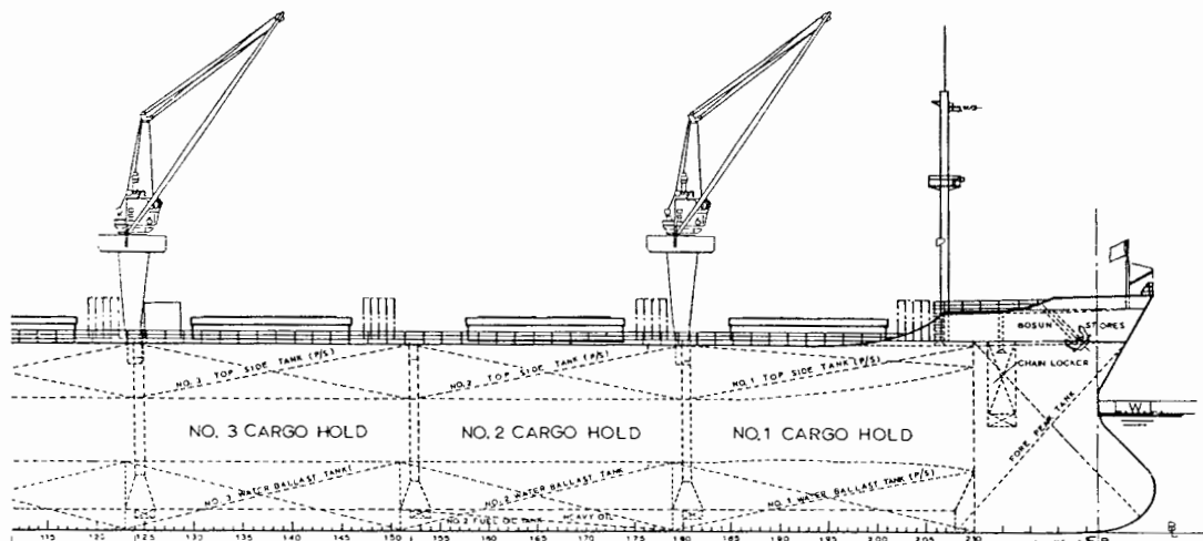
INBOARD PROFILE
