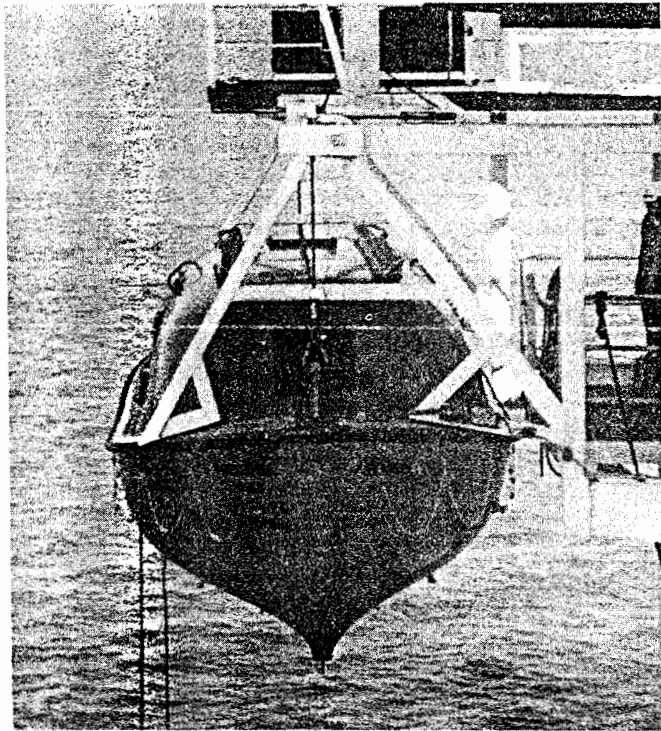
Fig. 27 Modern fire-protected covered lifeboat
