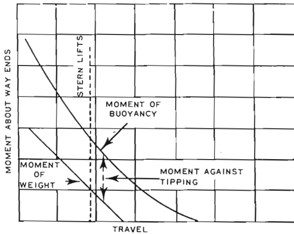
Fig. 13 Tipping curves
