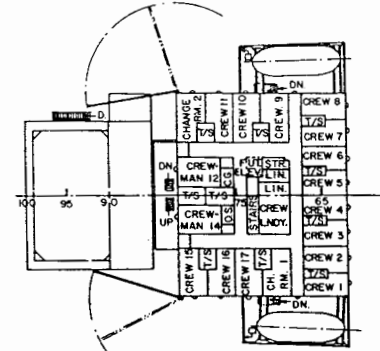
"A" DECK
