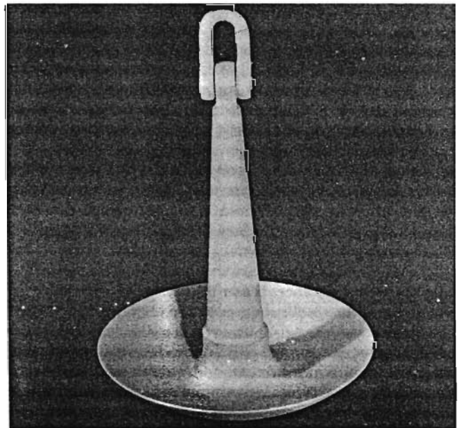
Fig. 13 Mushroom anchor
