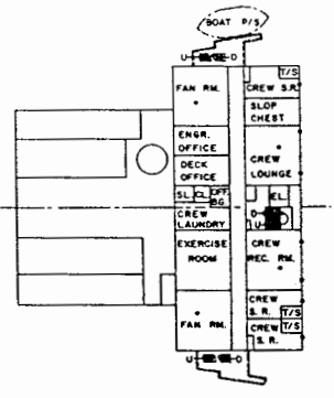
1ST LEVEL 5 CREW S.R.
