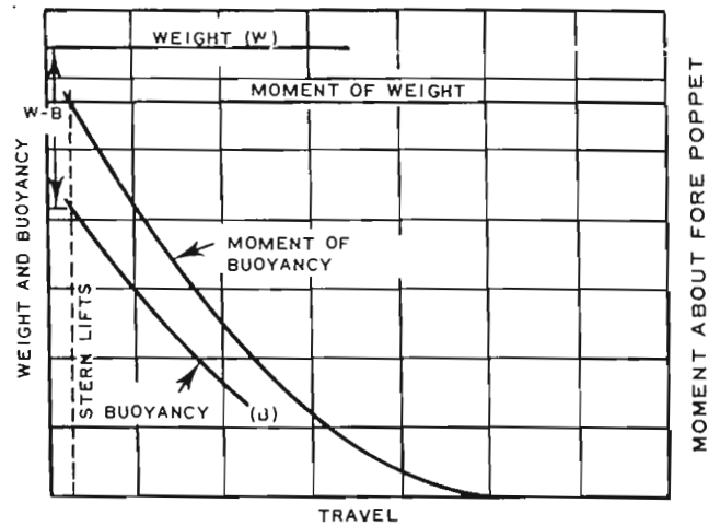
Fig. 14 Pivoting curves
