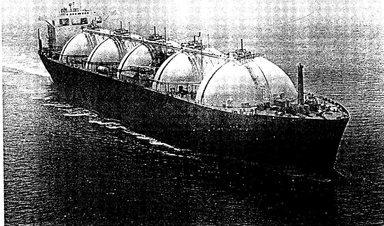
Fig. 4 SS LNG AQUARIUS—first Liquefied Natural Gas (LNG) tanker constructed in the United States at General Dynamics, Quincy Shipbuilding Division in 1977 for Energy Transportation Corporation; Molded dimensions 285.3 m (936 ft) by 43.7 m (143.5 ft) by 25 m (82 ft)
