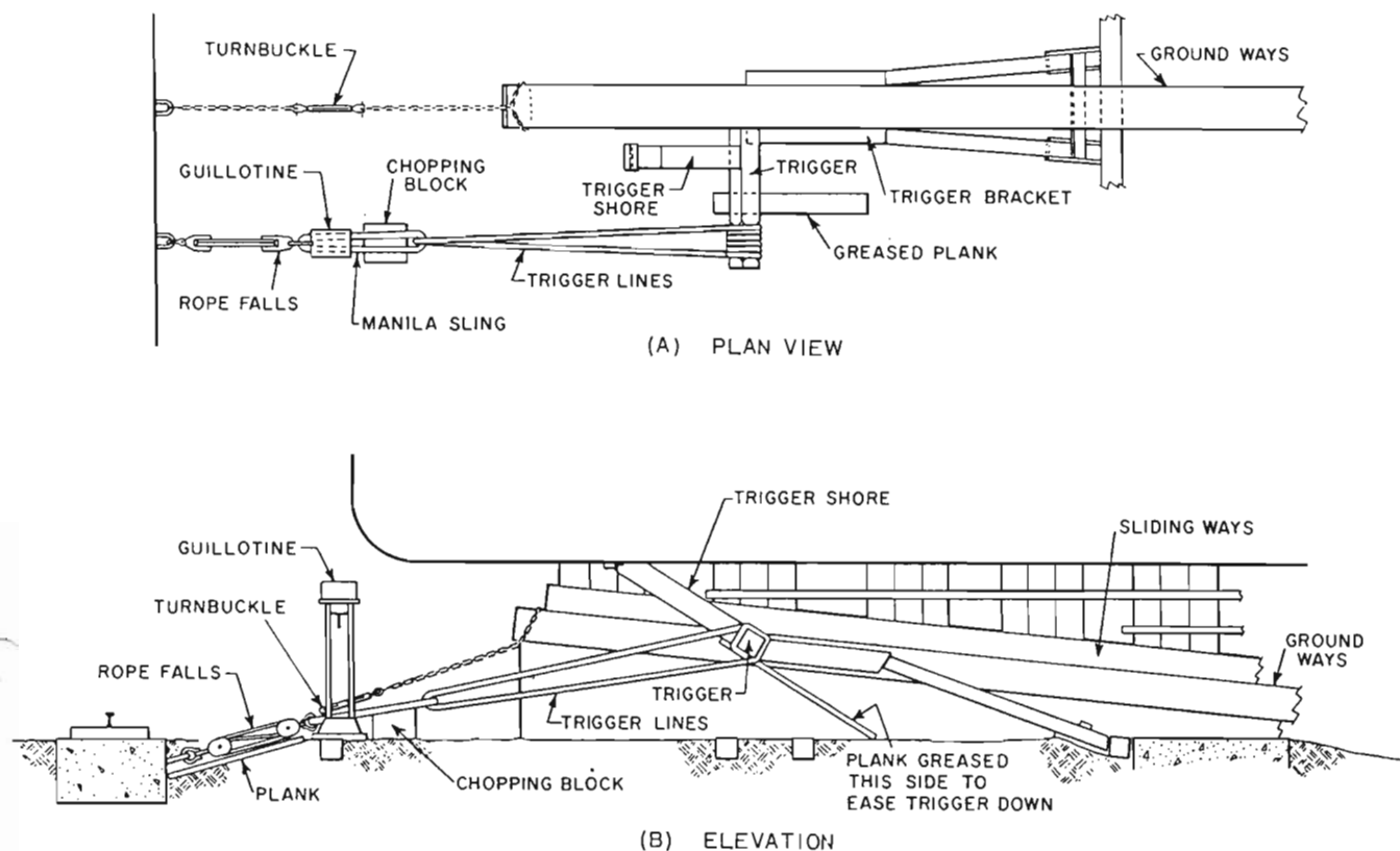
Fig. 12 Side launch trigger
