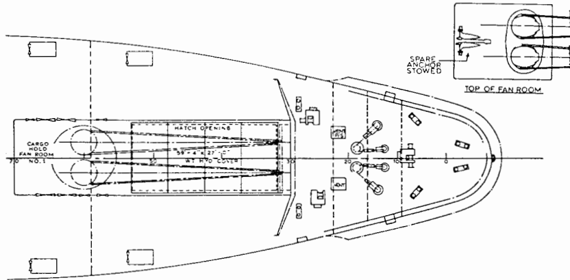
A DECK
