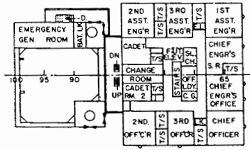
"B" DECK
