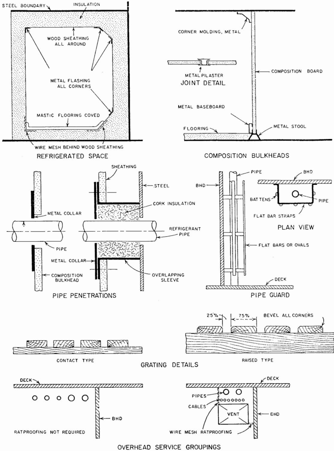
Fig. 23 Typical ratproofing details
