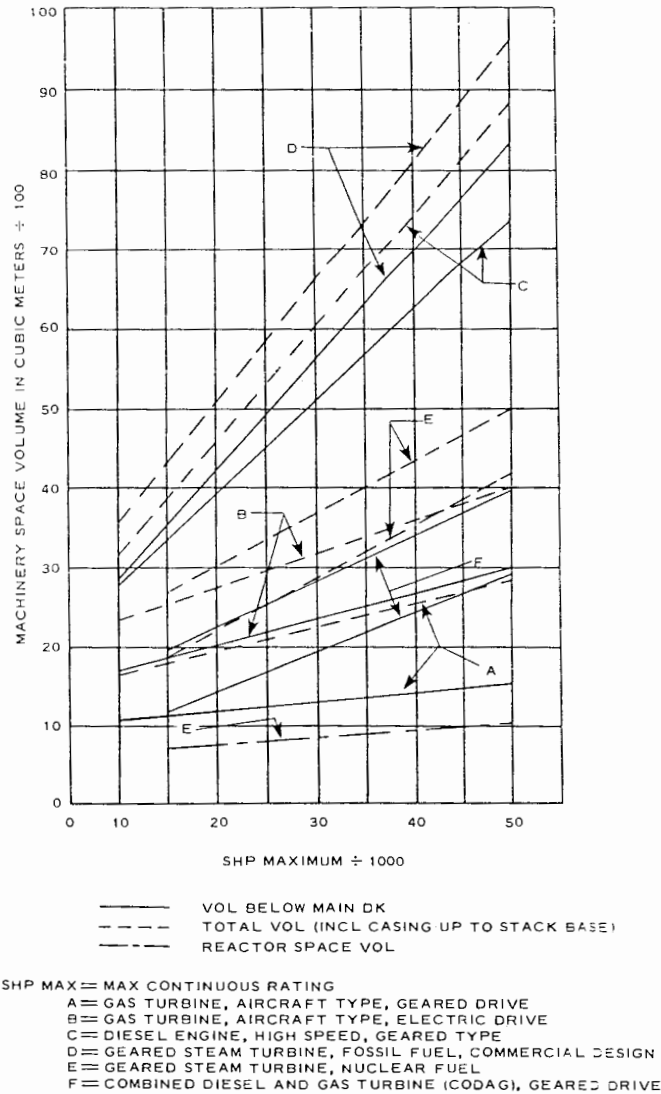
Fig. 6 Approximate volume of machinery space
