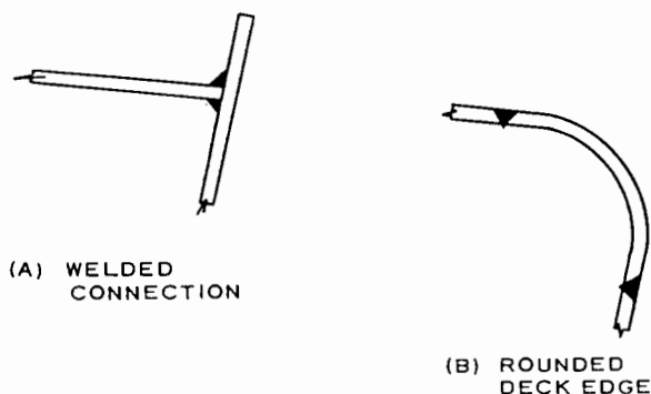
Fig. 25 Gunwale connections
