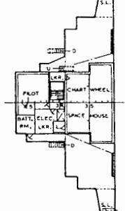
NAV. BRIDGE DK.
