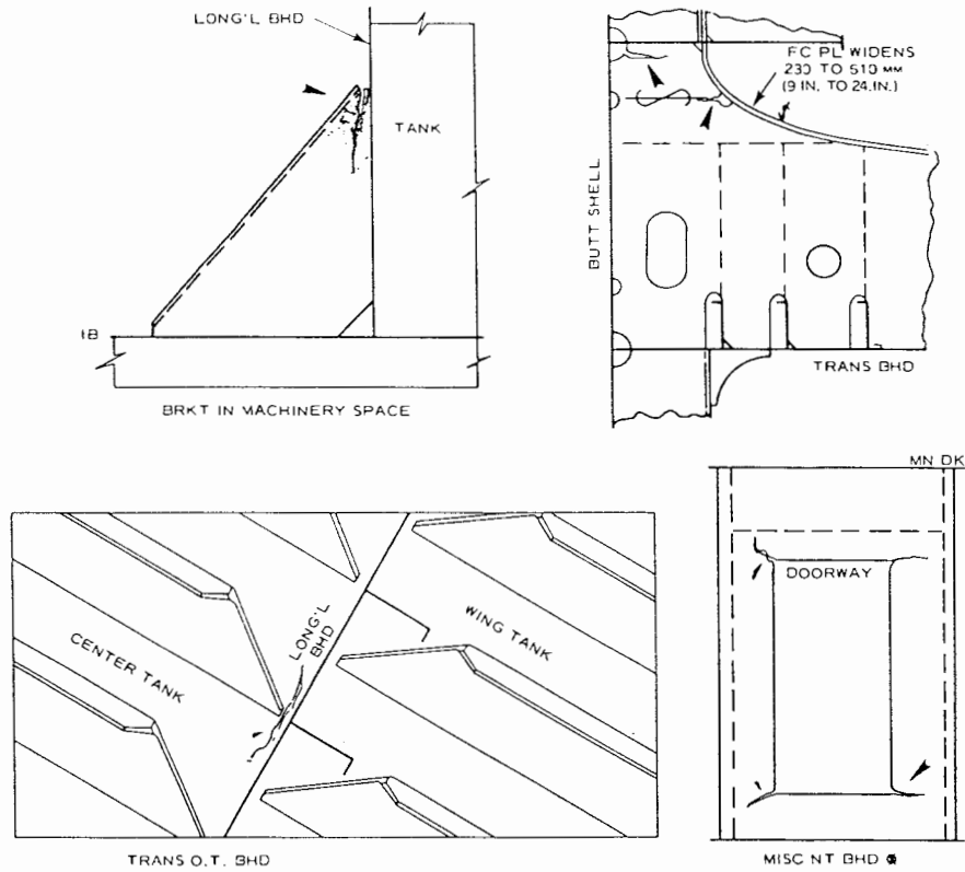
Fig. 16 Fatigue crack in areas of stress concentration
