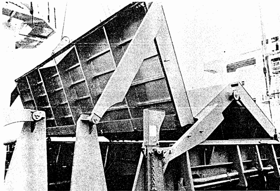
Fig. 9 Direct-pull weather deck hatch covers
