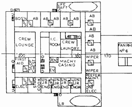
BOAT DECK
