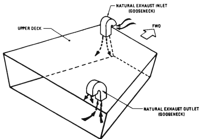
Fig. 1 Natural ventilation system
