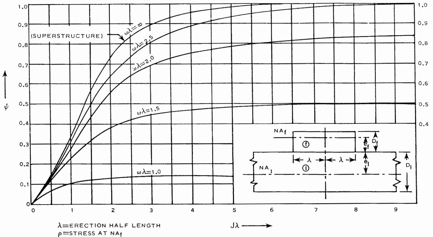
Fig. 43 Erection efficiency \psi
