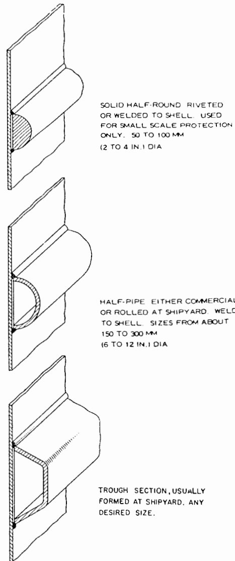
Fig. 85 Steel fenders
