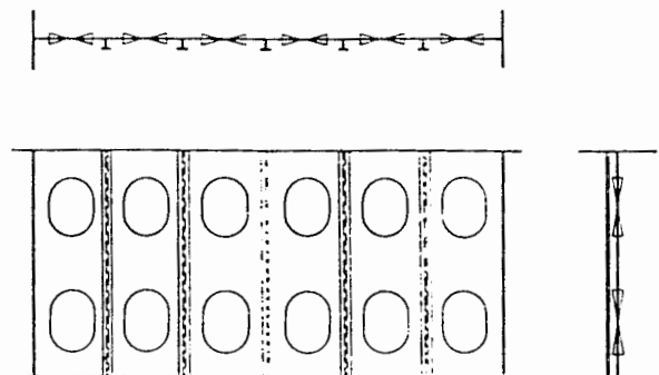
Fig. 42 Swash bulkhead
