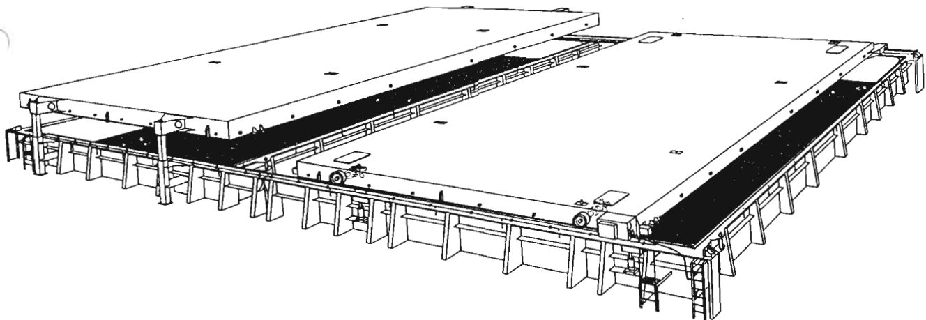
Fig. 43 Piggyback bulk carrier hatch cover
