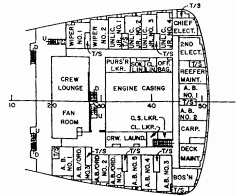
"A" DECK AFT
