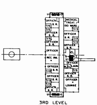
3RD LEVEL 8 OFFICER S.R.
