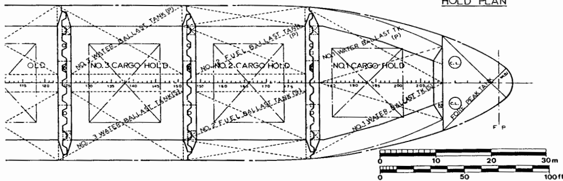
HOLD PLAN
