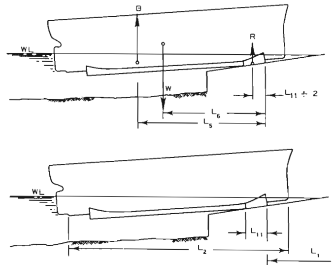
Fig. 20 Vessel pivoting
