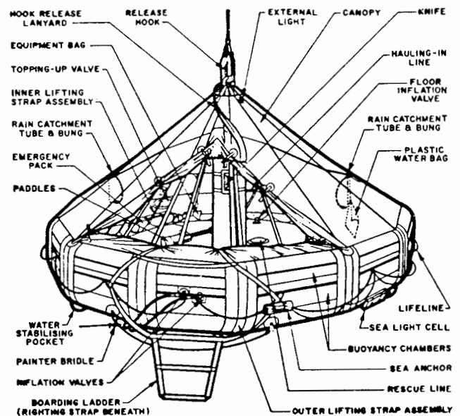
Fig. 28 Typical davit raft
