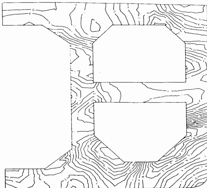
(C) STRESS CONTOURS
