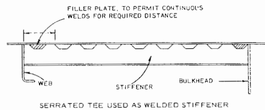
SERRATED TEE USED AS WELDED STIFFENER
