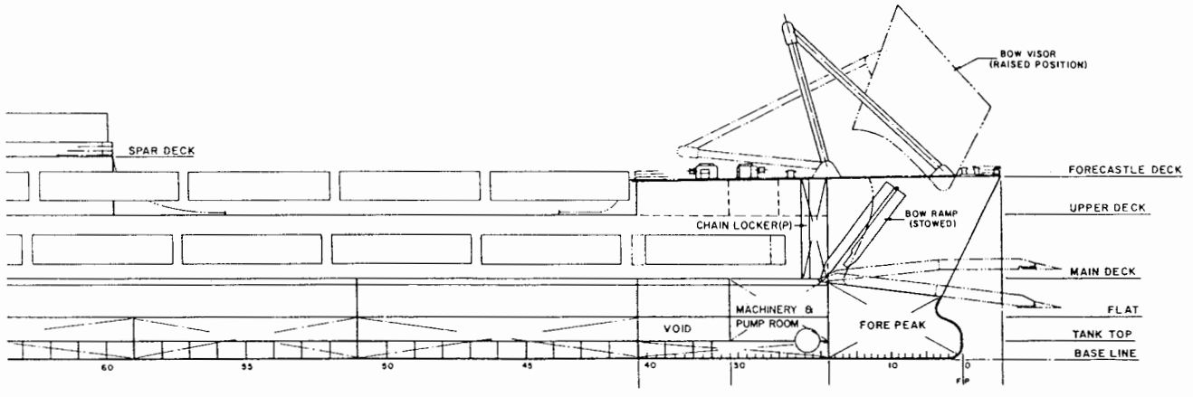
INBOARD PROFILE
