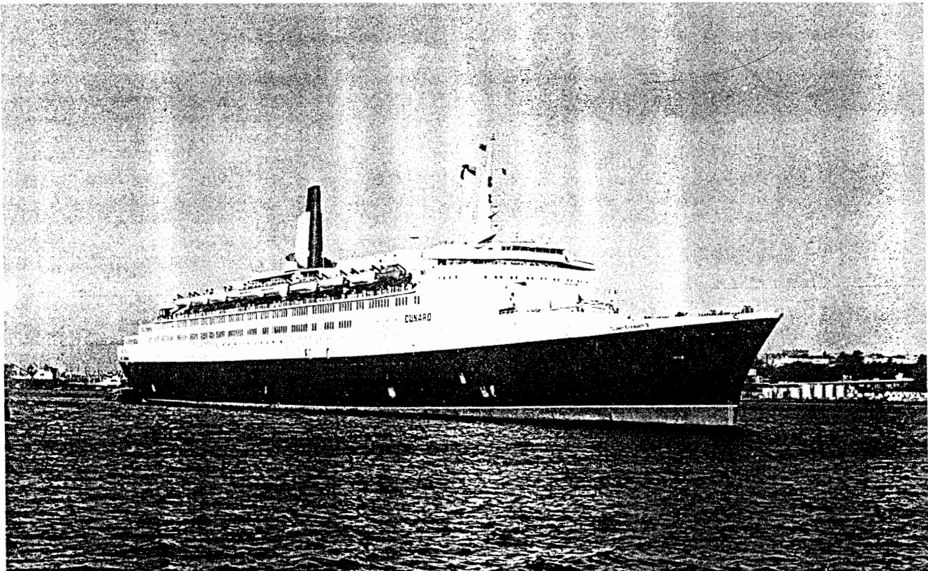
Fig. 9 SS QUEEN ELIZABETH 2—passenger liner built in 1969 at John Brown Shipbuilding Company for Cunard Line Ltd.; Molded dimensions 293.5 m (963 ft) by 32 m (105 ft) by 17.1 m (56 ft)
