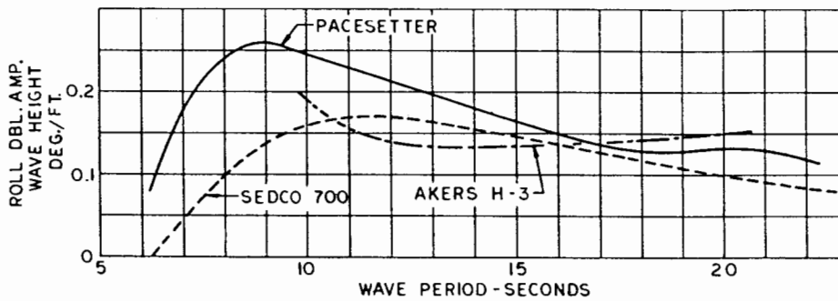
Fig. 37 RAO curves—pitch/roll
