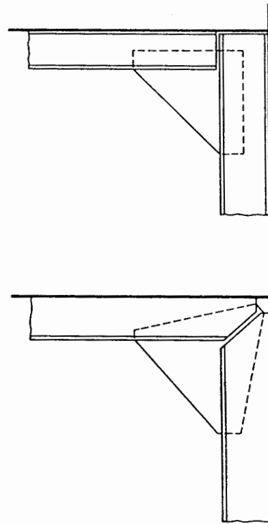
Fig. 32 Beam knees
