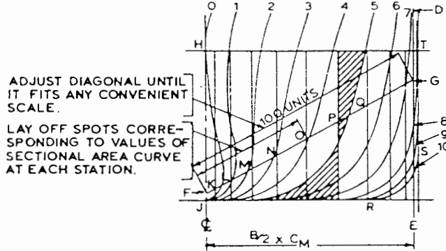
Fig. 25 Graphical aid to fair rough underwater body plan
