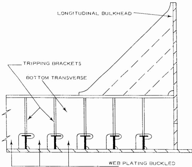
Fig. 7 Buckling of bottom transverse web frames
