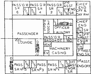
CABIN DECK
