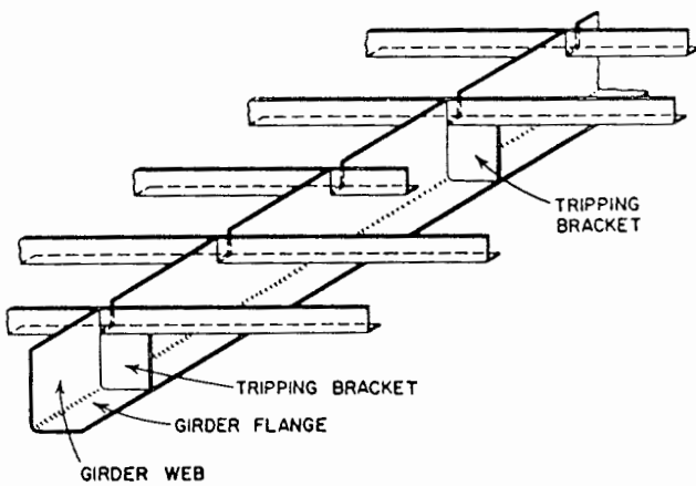
Fig. 54 Tripping brackets
