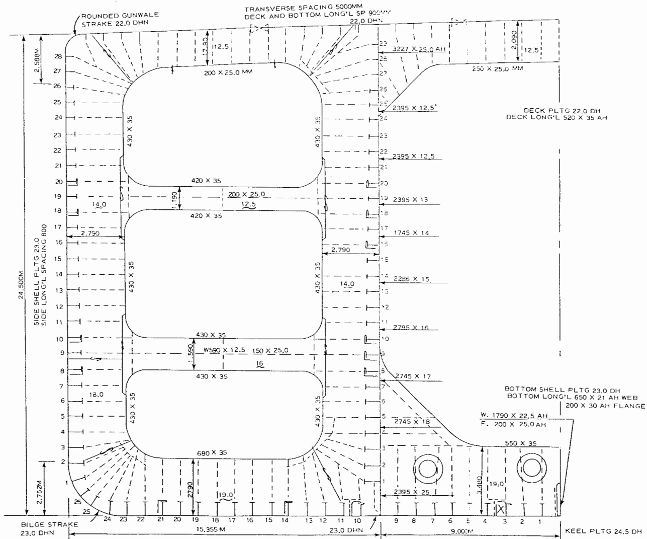
Fig. 49 Midship section designed based on ABS Rules 1980
