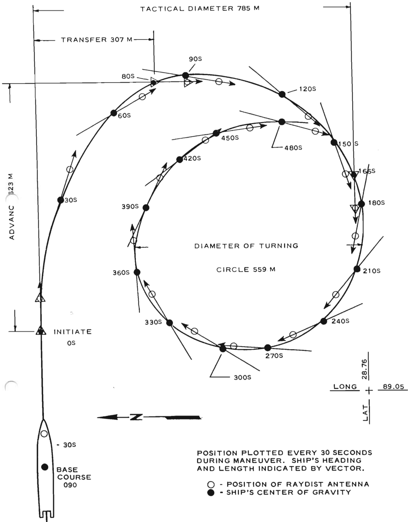
Fig. 2 Radiometric plot right turning circle
