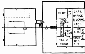
"C" DECK
