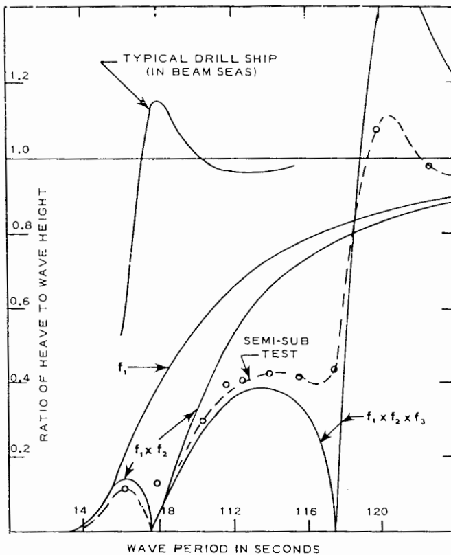
Fig. 35 Motion curves
