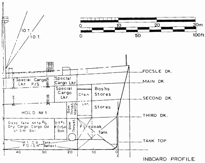
INBOARD PROFILE
