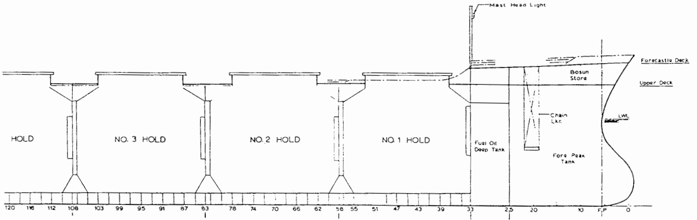
INBOARD PROFILE
